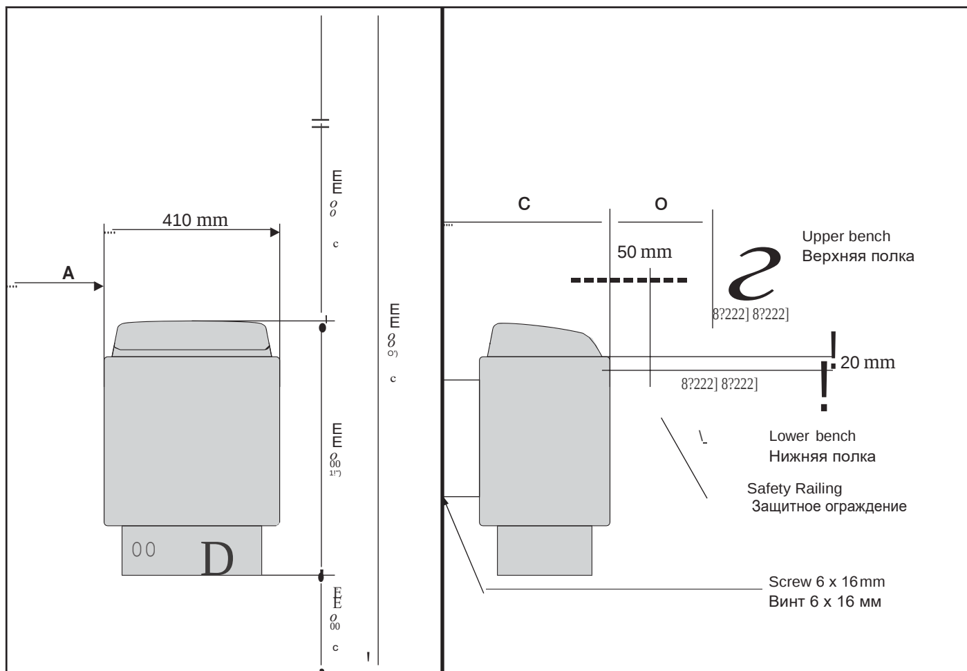
Fig. 6. Safety distances
