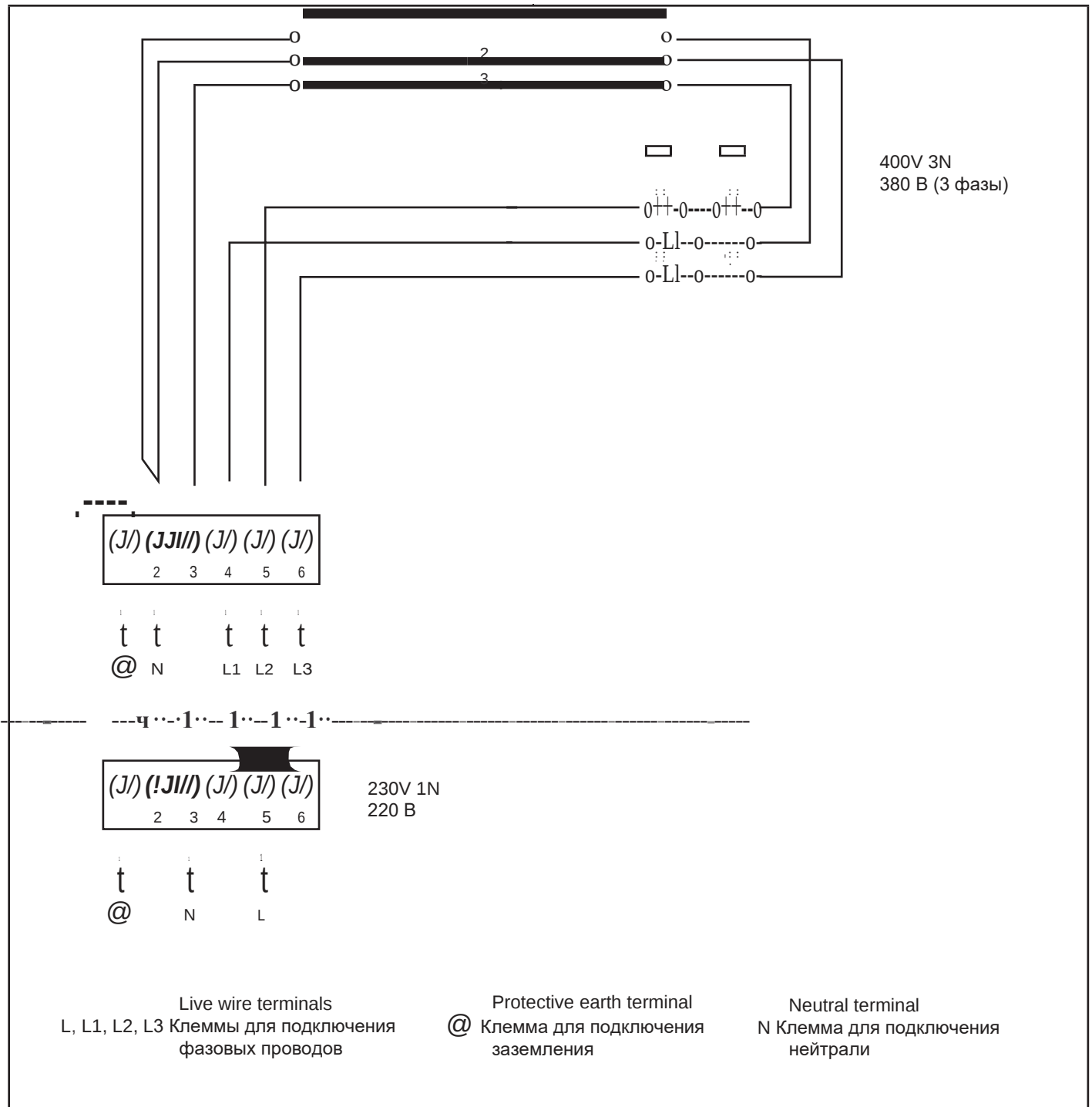
Fig. 7. Electrical connections
