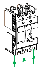
Reverse feeding.
