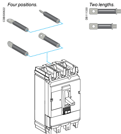
1-cable connector for EZC400/630.
